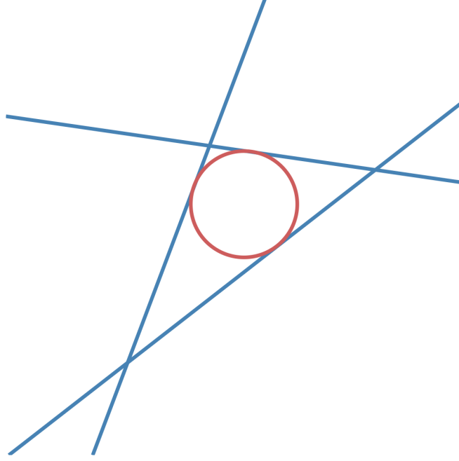
FIGURE 2. A red circle tangent to three blue lines that form a triangle. The proof of Theorem 2.2 considers such a triangle and finds a nearby arrangement of three hyperbolas, such that there are 136 real circles tangent to the three hyperbolas. In fact, the arrangement of hyperbolas in the proof of Theorem 1.3 is near the triangle shown in the picture.
