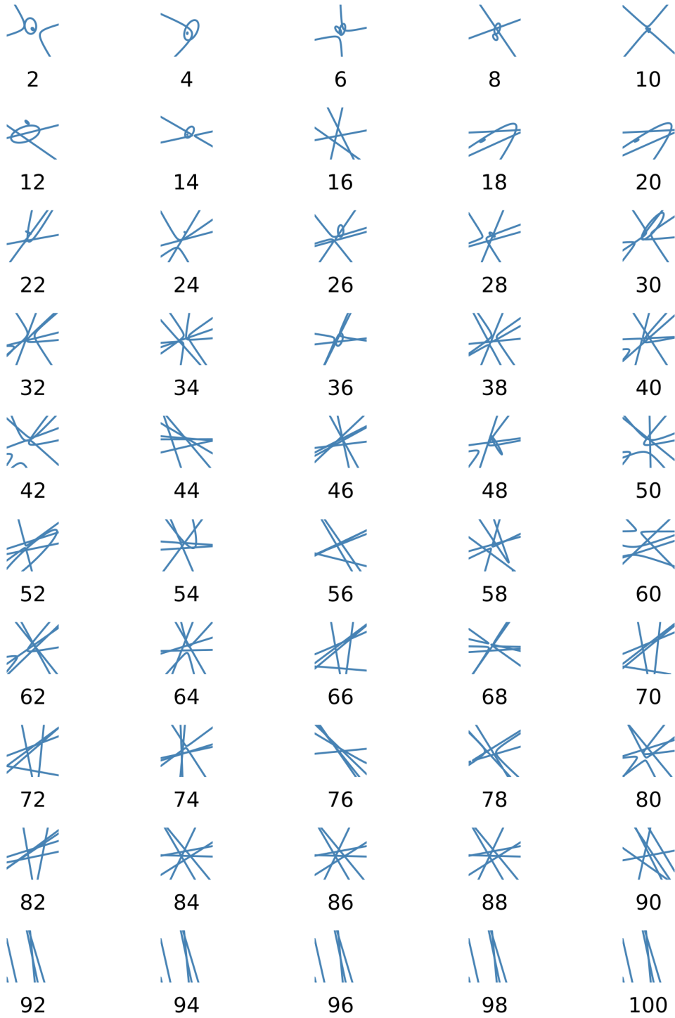
FIGURE 3. We show the first 50 conic arrangements that were used to prove Theorem 3.1. The number below each plot indicates the number of real tritangent circles. Starting from 92 real circles the arrangement all look similar to a triangle as in Figure 2.
