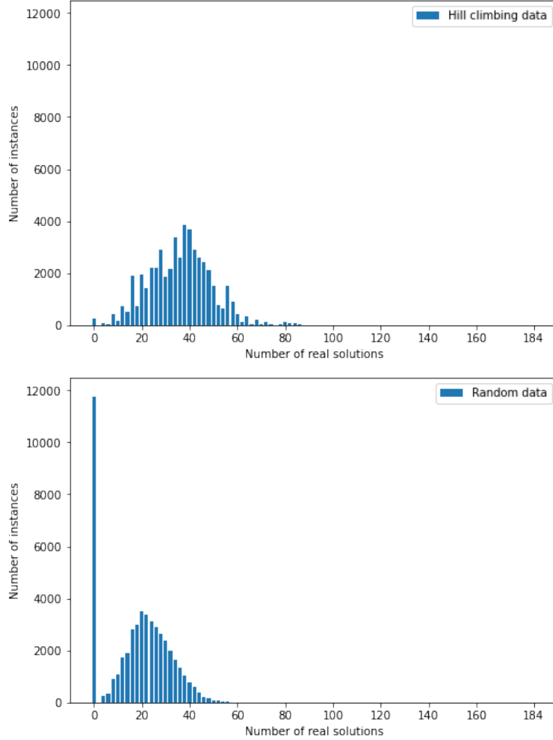
FIGURE 4. Two histograms showing the distribution of the number of real circles tangent to a given configuration of conics. The top histogram shows the distribution on the data \mathcal{D}_1 we generated using the hill climbing algorithm and the bottom histogram shows the distribution on random data \mathcal{D}_2 .
