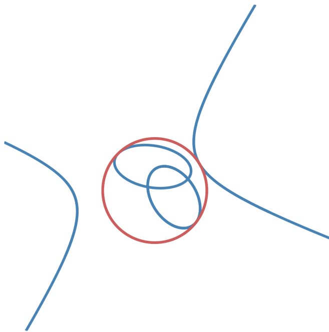
FIGURE 1. A red circle tangent to one blue hyperbola and two blue ellipses.
