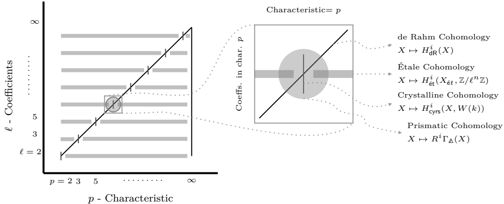
FIGURE 2. Prismatic cohomology at the (p, p) -point.
